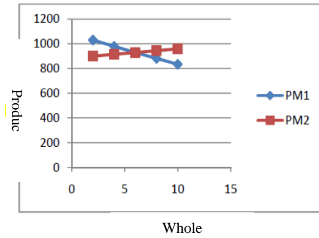
Fig. 5. Analysis of producer profit sensitivity to c1 change in wholesale Stackelberg.
