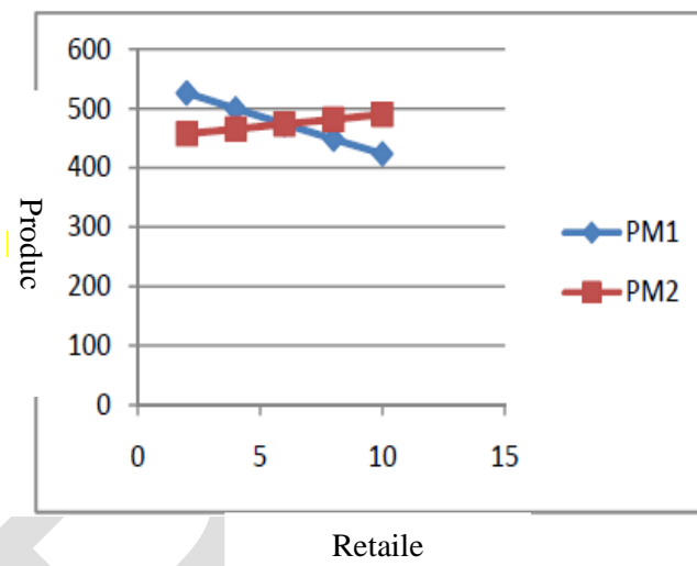
Fig. 6. Analysis of producer profit sensitivity to c1 change in retailer Stackelberg.
