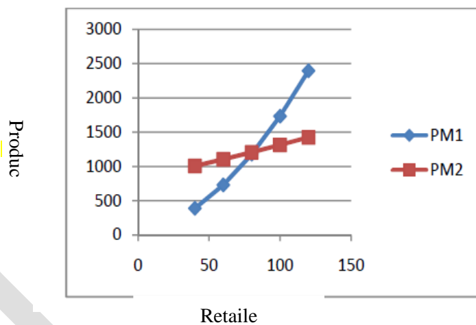
Fig. 4. Analysis of Sensitivity of producer profit to a_1 change in retail Stackelberg.
