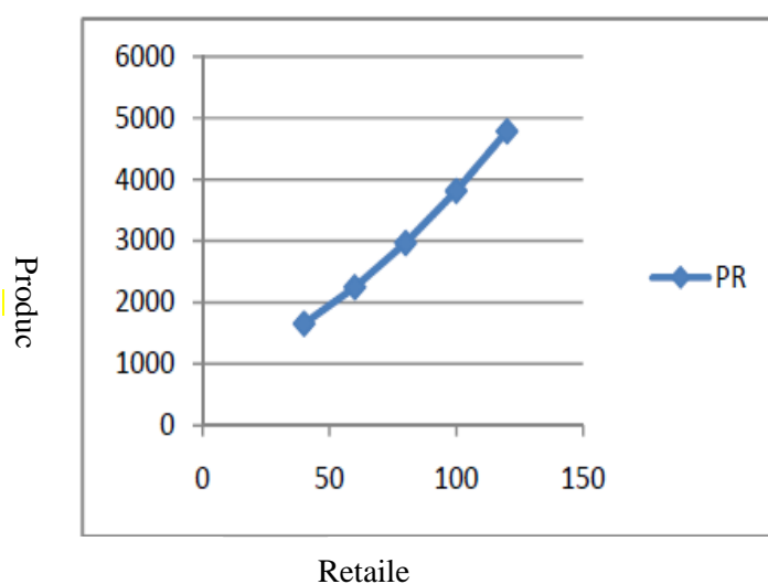
Fig. 8. Analysis of producer profit sensitivity to a1 change in retail Stackelberg.
