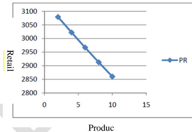
Fig. 10. Analysis of retail profit sensitivity to c_1 change in producer Stackelberg.
