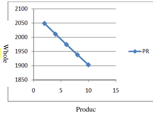
Fig. 9. Analysis of wholesale profit sensitivity to c_1 change in producer Stackelberg.
