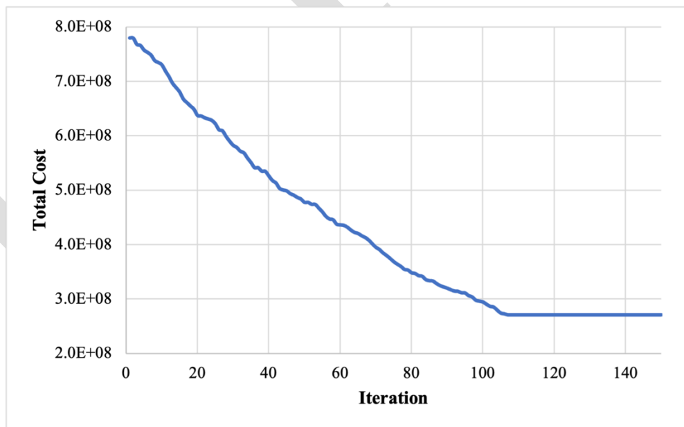
Fig. 5. Convergence of ICA in test problem
