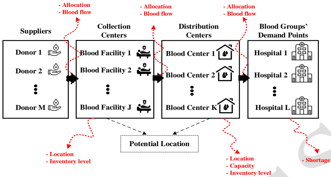
Fig. 1. Problem configuration
