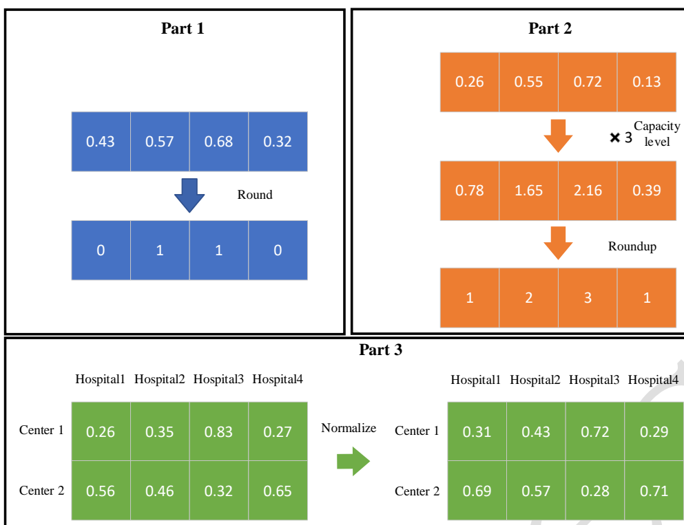
Fig. 4. Solution representation
