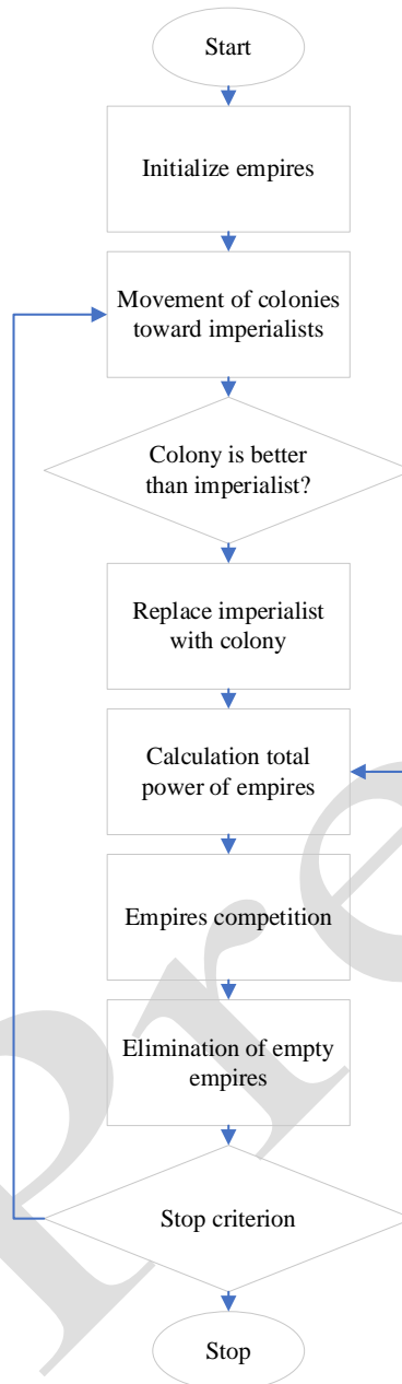
Fig. 3. ICA flowchart
