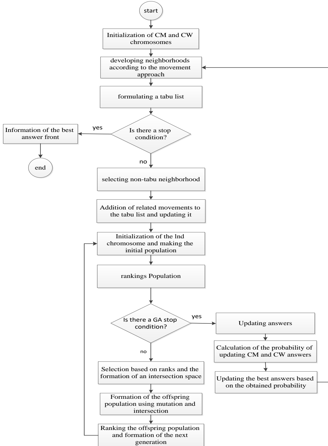
Fig. 1. Flowchart of MO-TS-GA hybrid algorithm.
