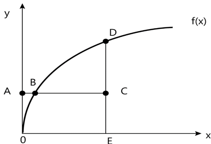
Figure 1 - Representation of the Efficiency Border resulting from the use of the DEA.
