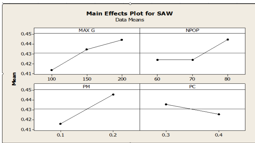
Fig. 4. Minitab software output to determine the parameter of the NSGA-II algorithm.
